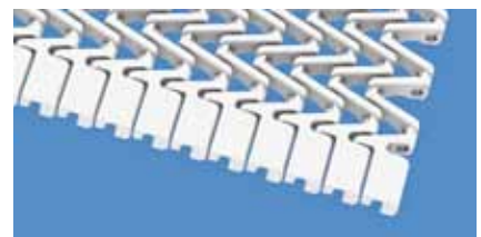
S15 | 47% open | Reduced surface area
